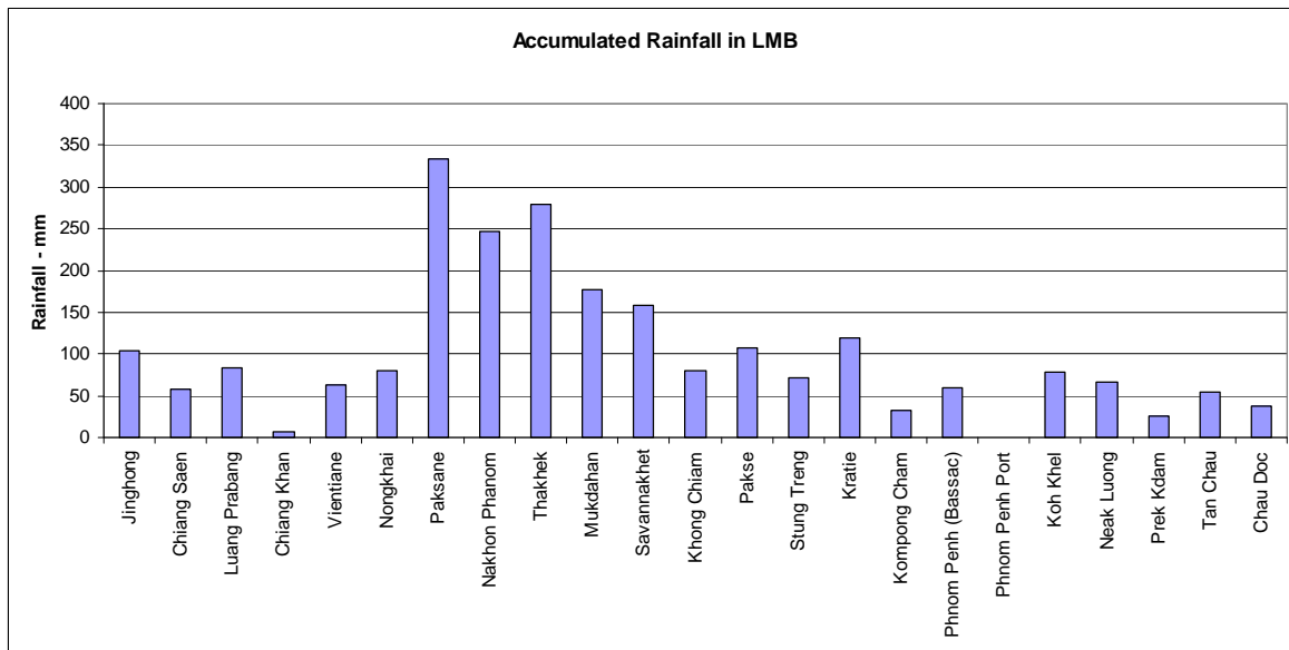
Figure 1: Accumulated Rainfall Distribution over the LMB from 03 rd – 10 th July 2017
