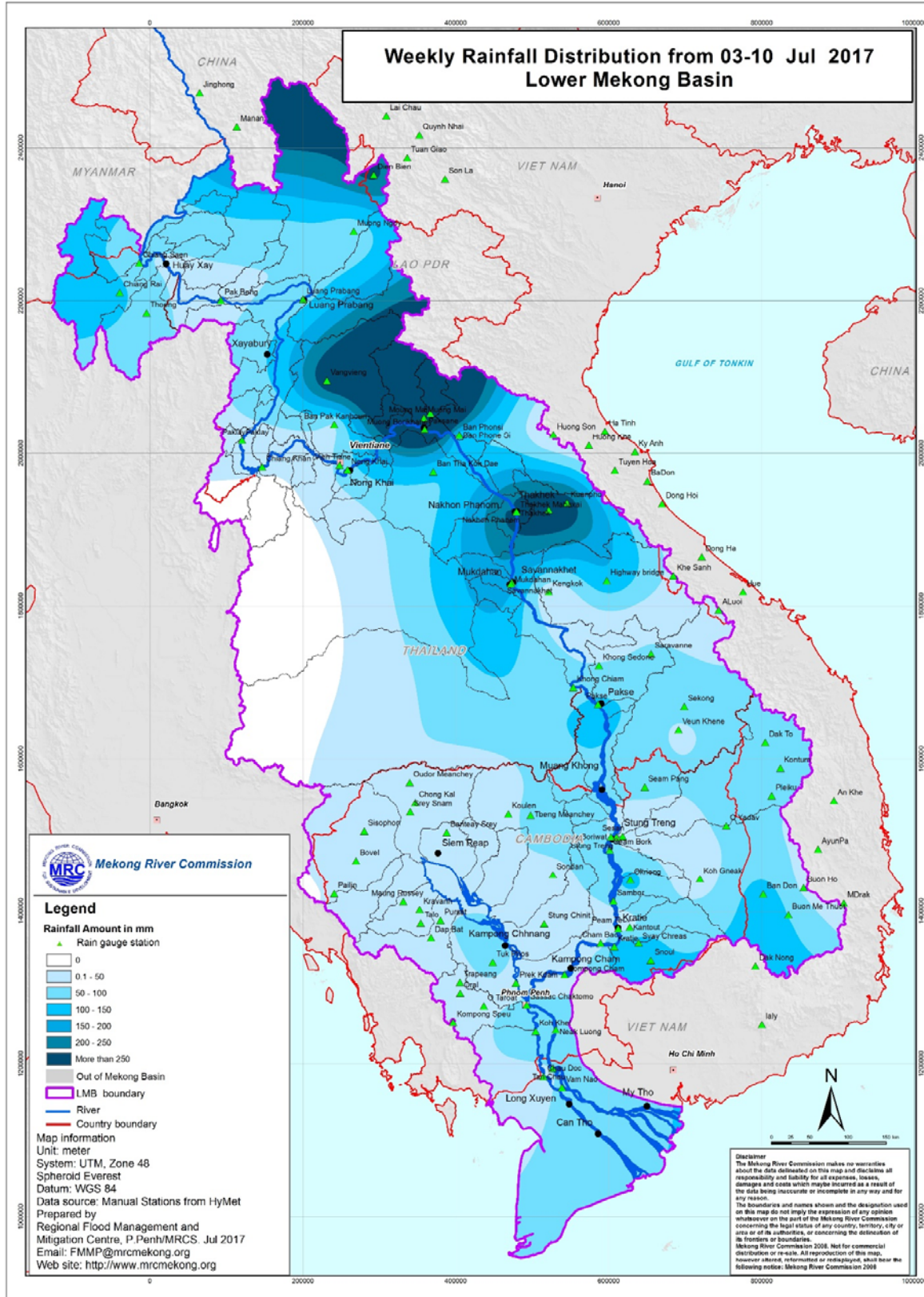
Figure 2: Weekly Rainfall Distribution over the LMB from 03 rd – 10 th July 2017
